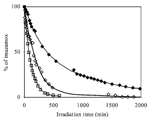
Figure 3. Degradation kinetics for 10 \text{ mg L}^{-1} imazamox without metal salts ( \square ) and in the presence of \text{CaCl}_2 ( \diamond ) or \text{CuCl}_2 ( \blacklozenge ); pesticide to metal salt molar ratio R = 1 .
