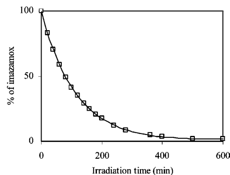
Figure 1. Photodegradation of imazamox (○, 10 mg L -1 ) in deionized water followed by LC-DAD.
