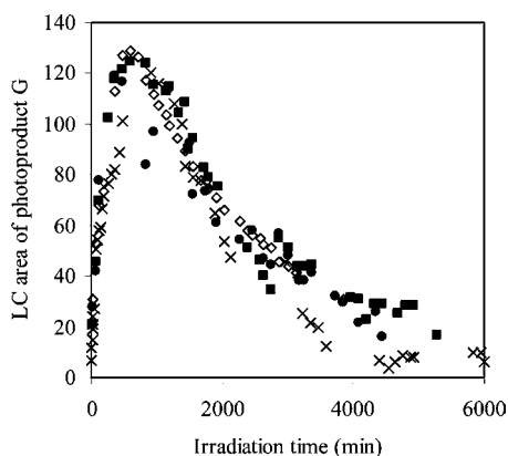
Figure 6. Degradation kinetics of photoproduct G in the presence of calcium salts: CaCl 2 (×) or Ca(NO 3 ) 2 (●) with R = 1 and CaCl 2 (■) or Ca(NO 3 ) 2 (◇) with R = 2 .
