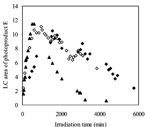
Figure 5. Degradation kinetics of photoproduct E for 10 mg L -1 imazamox without metal salts (▲) and in the presence of Ca(NO 3 ) 2 (◇) or Cu(NO 3 ) 2 (◆) with R = 2 .
